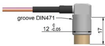
T3-FL-M1205-KR (flange version)
