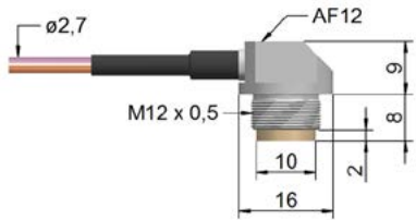
T3-FL-M1205-KR (flange version)
