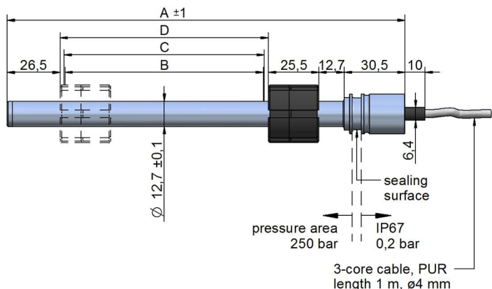
LMI12-SE with standard flange
