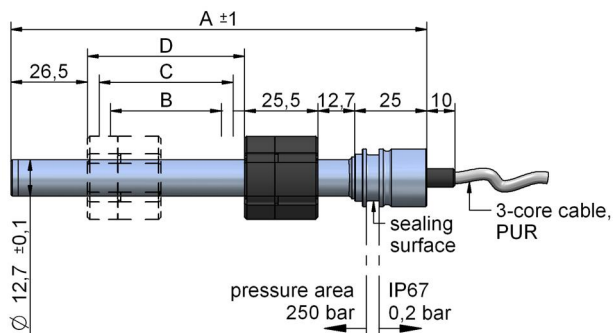
LMI12-SL with standard flange
