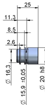
Detail drawing standard flange
