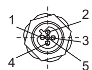
Corresponding mating connector: 05.BMSWS 8151-8.5
